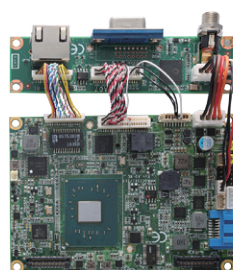
▲ Assembly view
