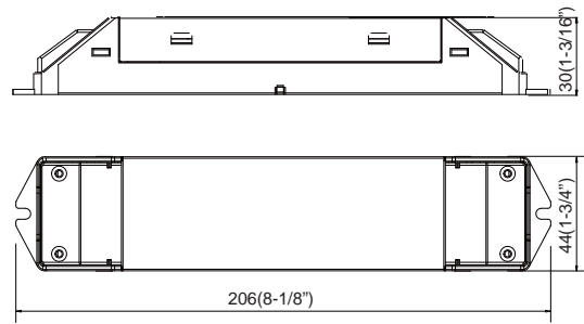
Dimensions:(mm/inches)
