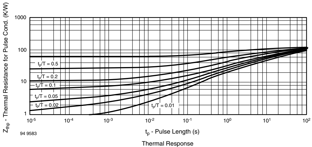
Thermal Response
