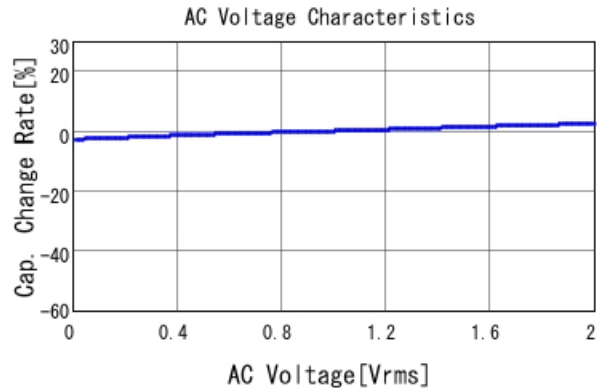
GCM188R71H104KA57 C-AC Voltage capchange, DCOV, 25
