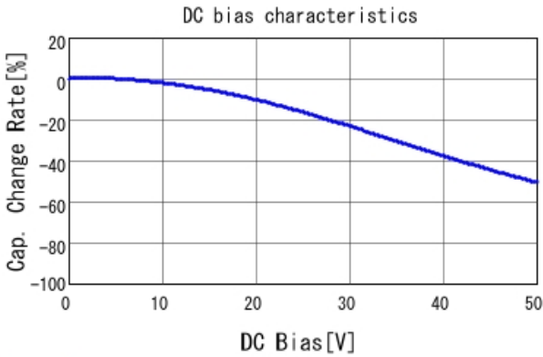
GCM188R71H104KA57 C-DC bias capchange, 25.0degC, A
