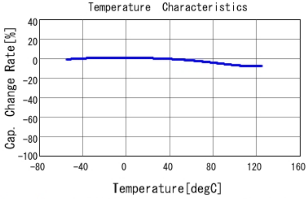
GCM188R71H104KA57 C-Temp. capchange, DC0.0V, AC1.C
