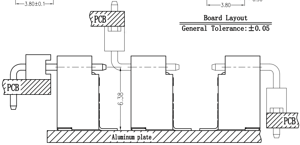
Assembly Layout
