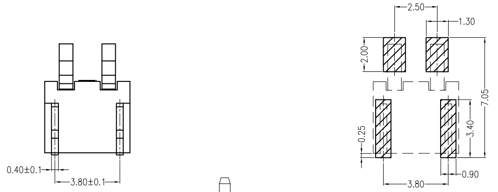
Board Layout General Tolerance: ±0.05
