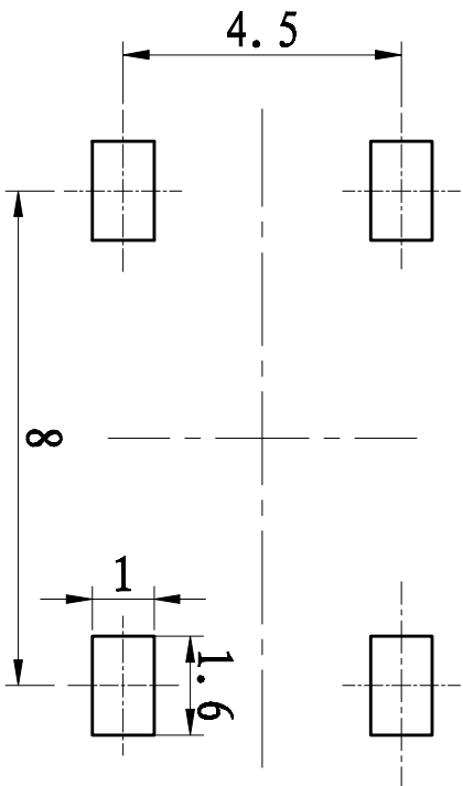
Suggested P.C.B Layout
