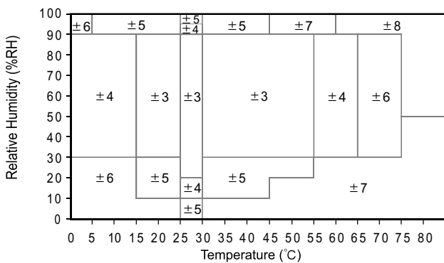
Figure 5 Maximum humidity error between 0~80 °C, unit: (% RH)
