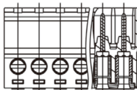
Section B-B
