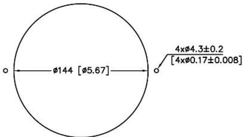
Mounting Panel Cutout Outlet Side & Inlet Side
