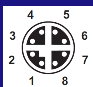
X-Coding M12
