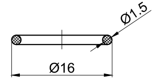
Seal Ring
