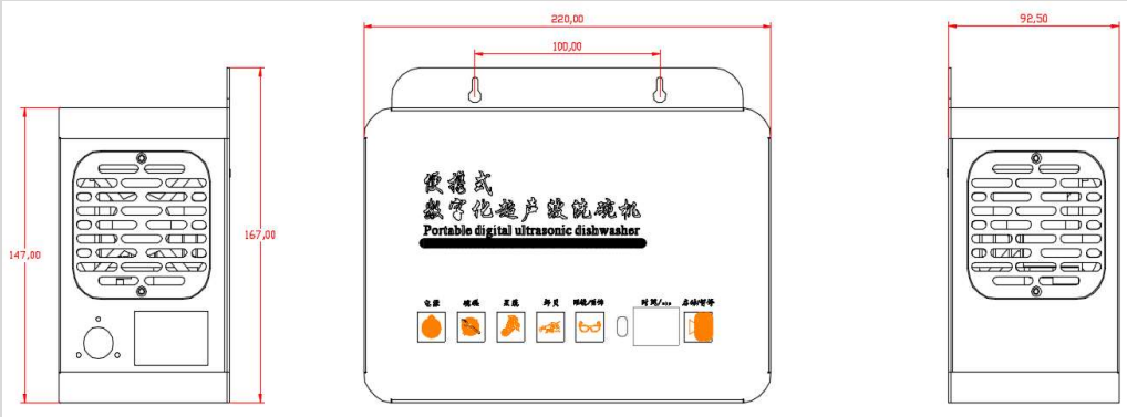
Installation Dimension
