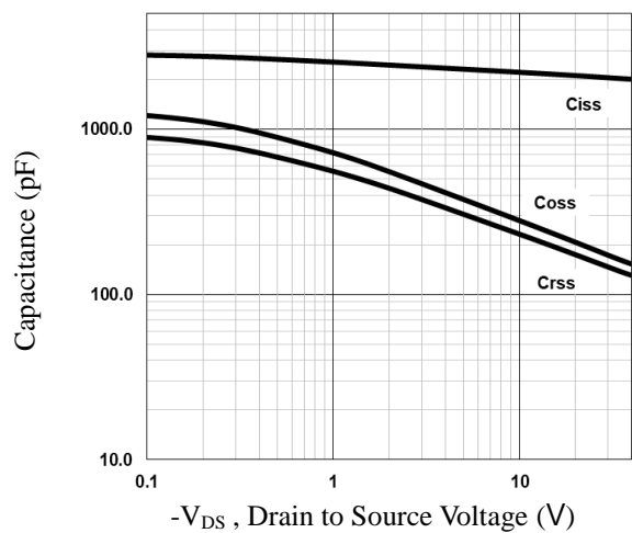
Fig.6 Capacitance Characteristics
