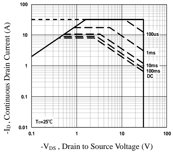
Fig.24 Maximum Safe Operation Area
