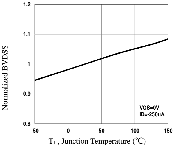
Fig.21 Normalized BVDSS vs. T_J
