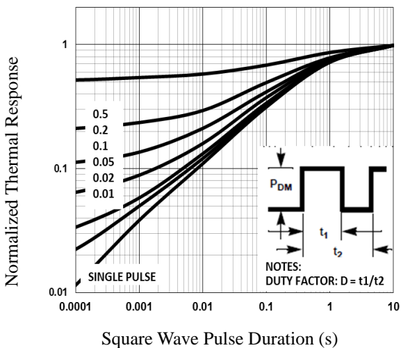
Fig.23 Normalized Transient Impedance
