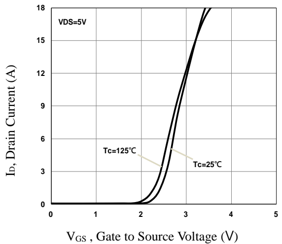
Fig.10 Transfer Characteristics
