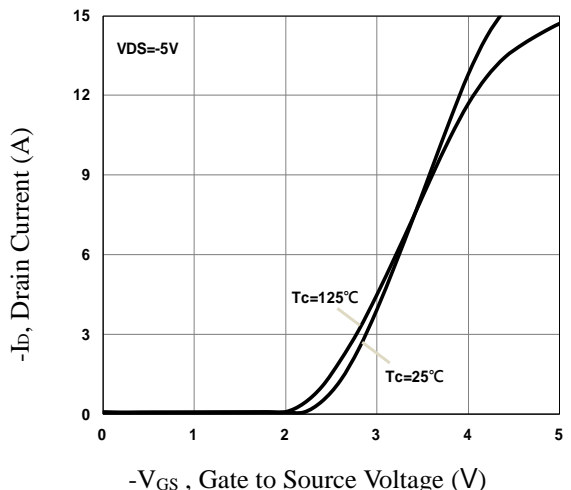
Fig.22 Transfer Characteristics
