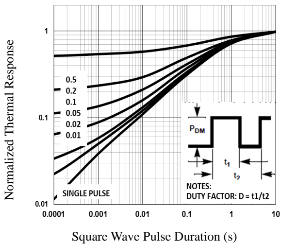
Fig.11 Normalized Transient Impedance
