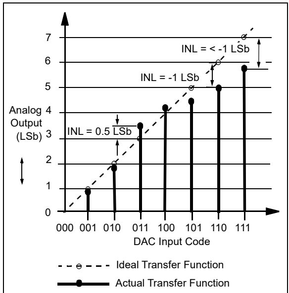
FIGURE C-4: INL ACCURACY.
