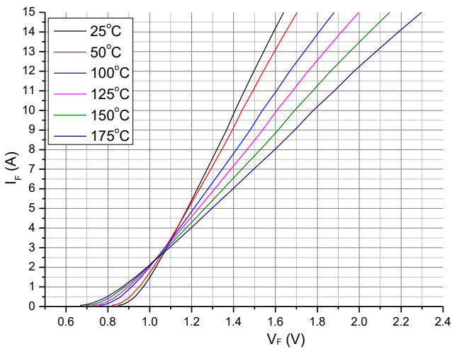
Fig.1-Forward Characteristics
