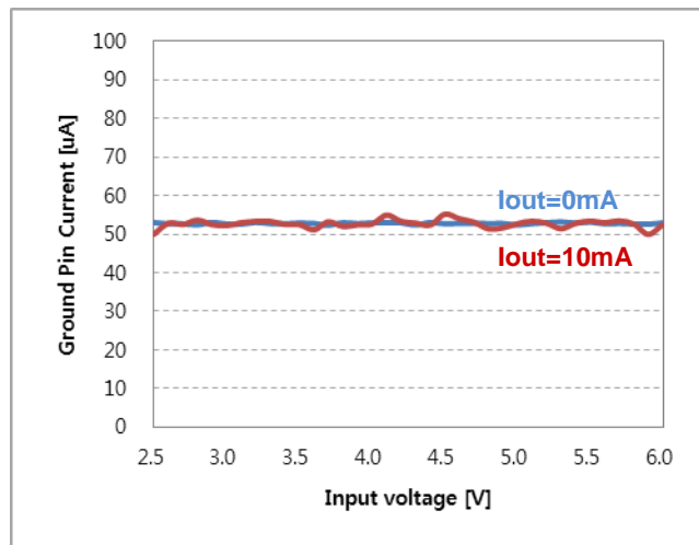
Ground Current @ I out =0A / 10mA (C in =10uF, C out =10uF, R 2 =36KΩ, R 1 =35KΩ)
