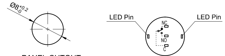
PANEL CUTOUT MAX.PANEL THICKNESS 6 mm
