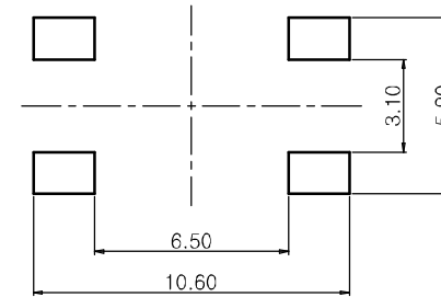
PCB DIMENSION
