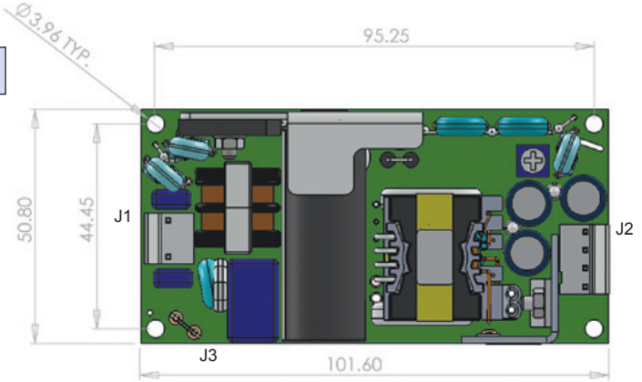
Outline Drawing ZMS100 24 - 48V Series
