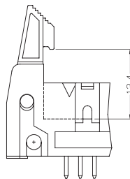
Short Lever
