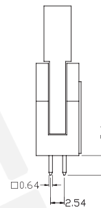
Straight Type
