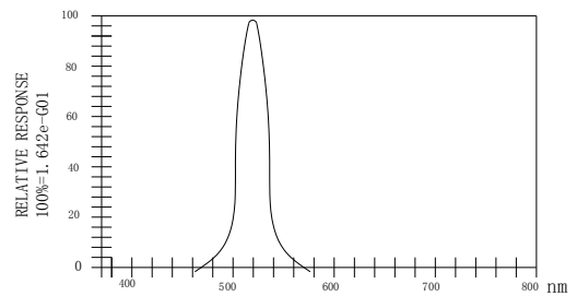
Luminous Spectrum (Ta=25°C) SPECTRAL RADIANCE
